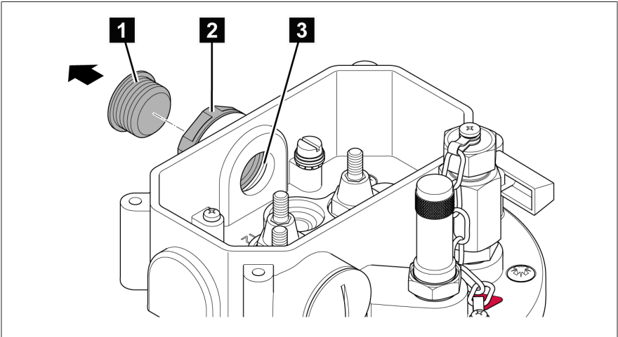
Figure 9: Dummy plug and M20/M25 adapter
