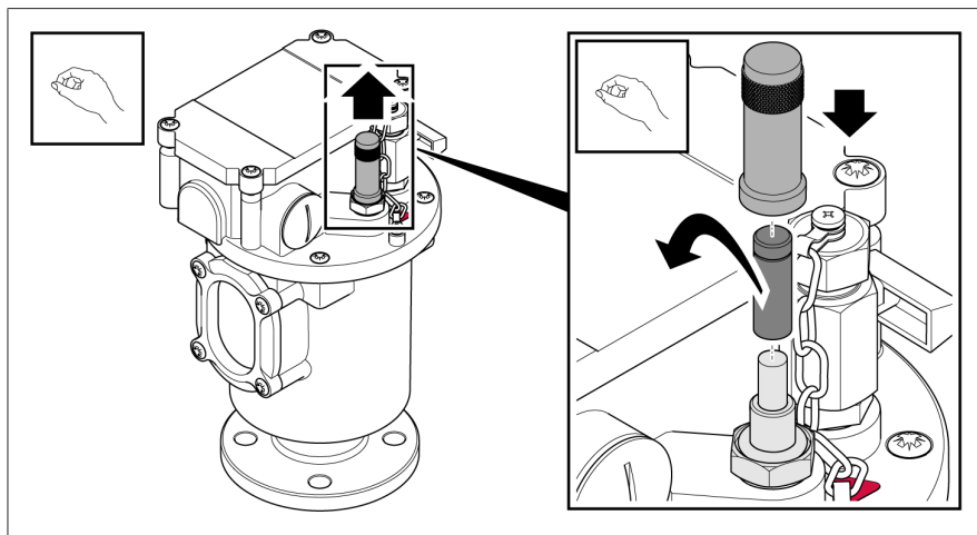
Figure 6: Removing the plug in the test button
