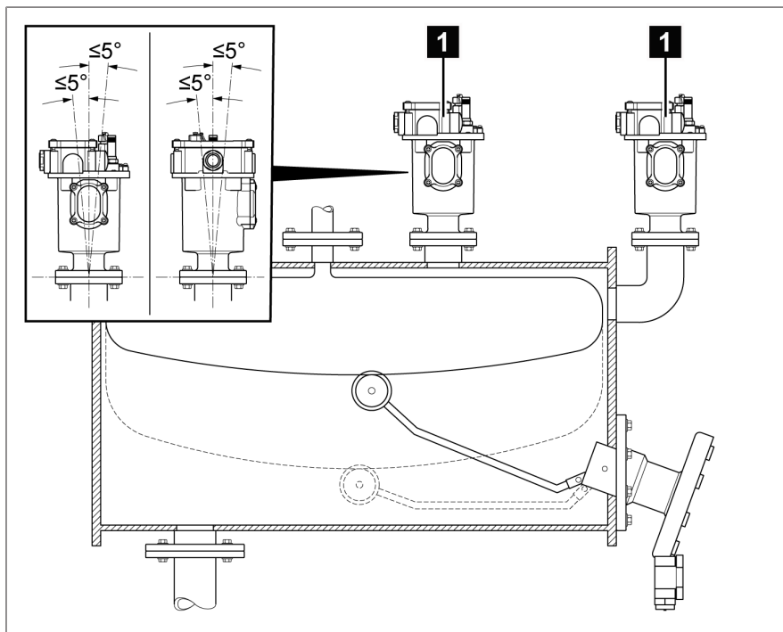
Figure 4: Permissible inclination of the protective relay
