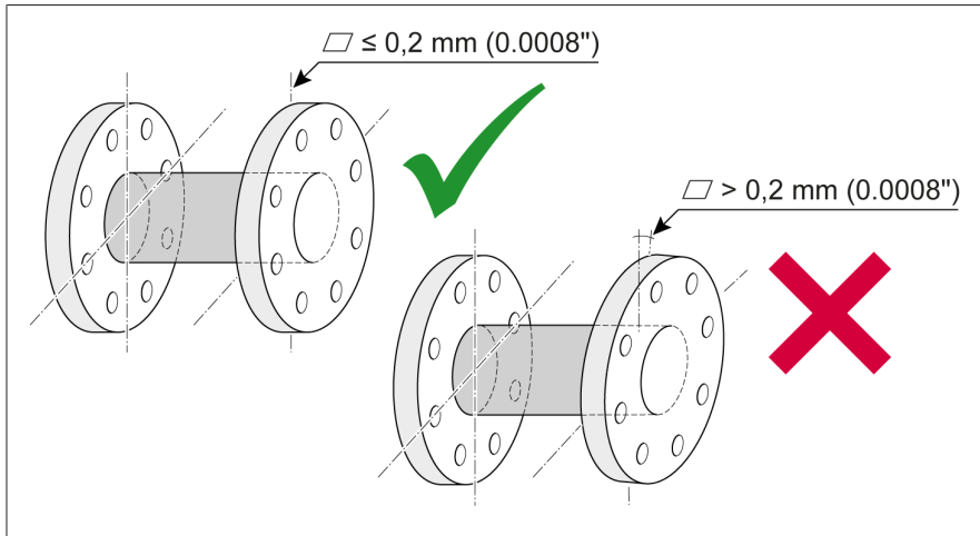
Figure 3: Flanges
