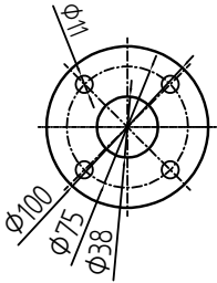
Detail of connecting flange
