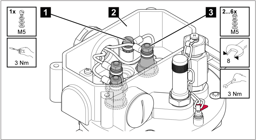
Figure 11: Terminal box
