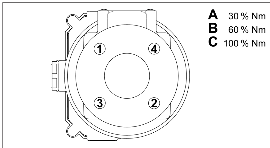
Figure 8: Tightening the screws crosswise
