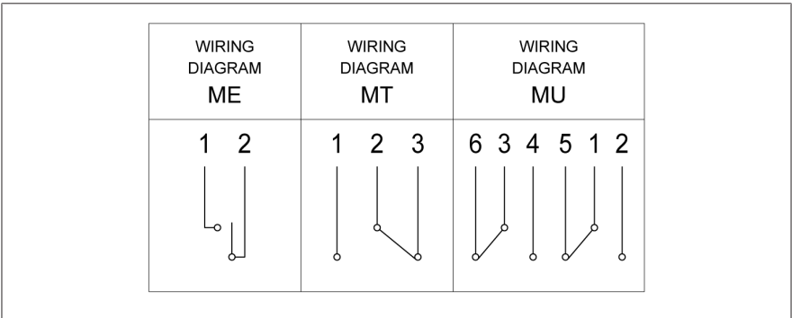
Figure 10: Wiring diagrams
