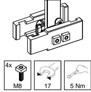
Bakelite movable contacts guide
