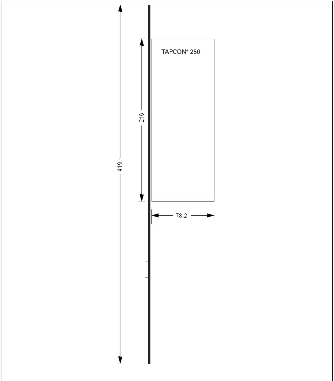
Figure 2 TC250-67 side view
