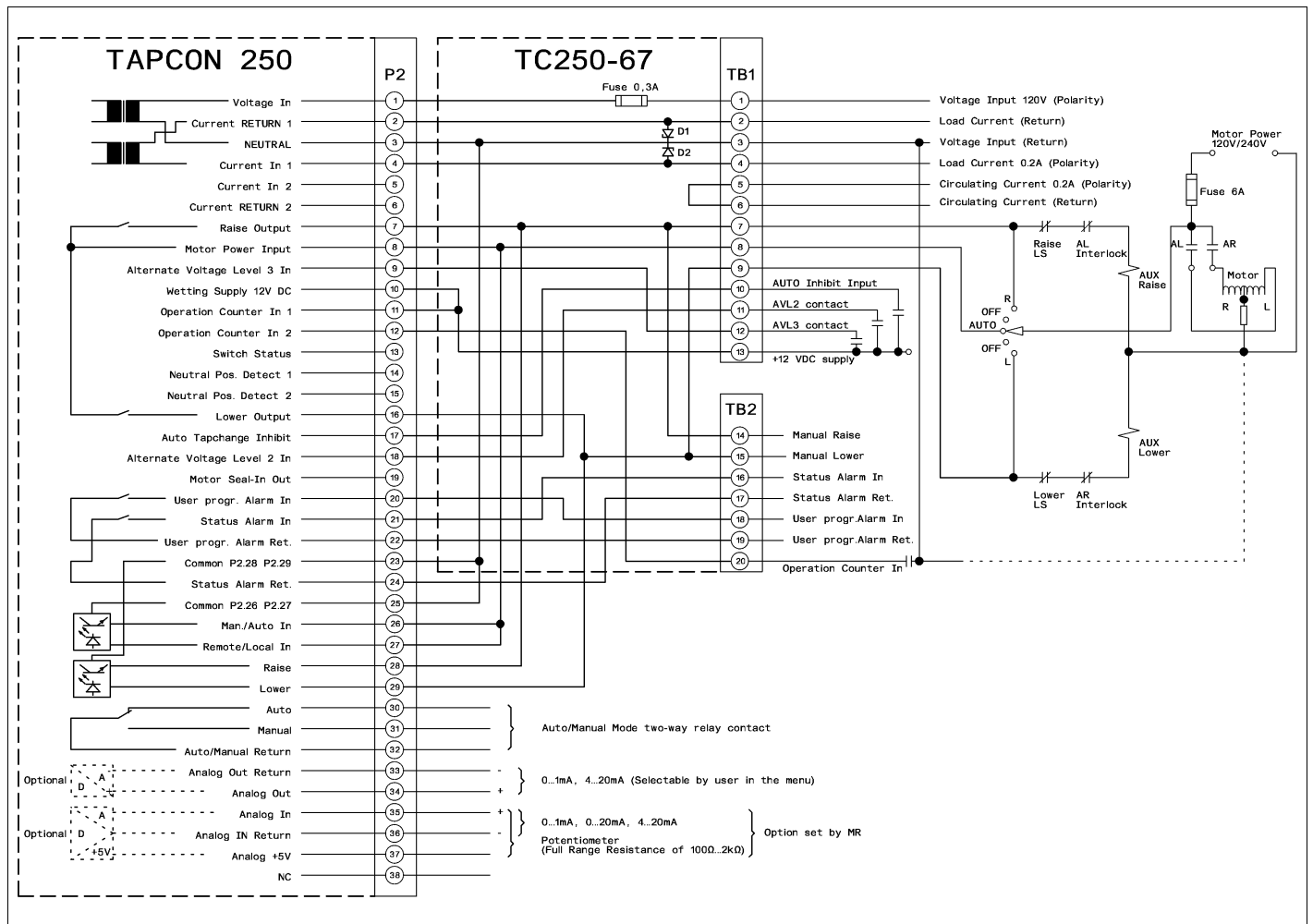
Figure 3 Wiring diagram
