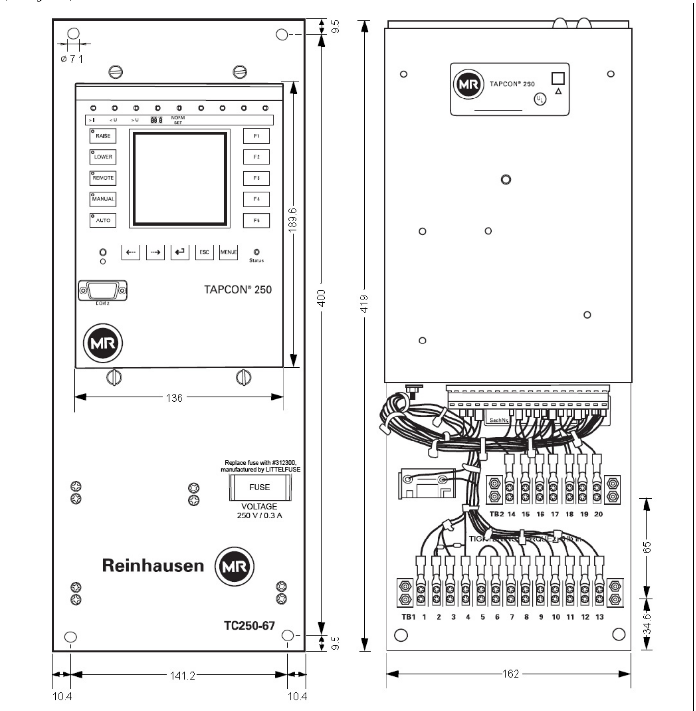
Figure 1 TC250-67 outline dimensions and rear view
